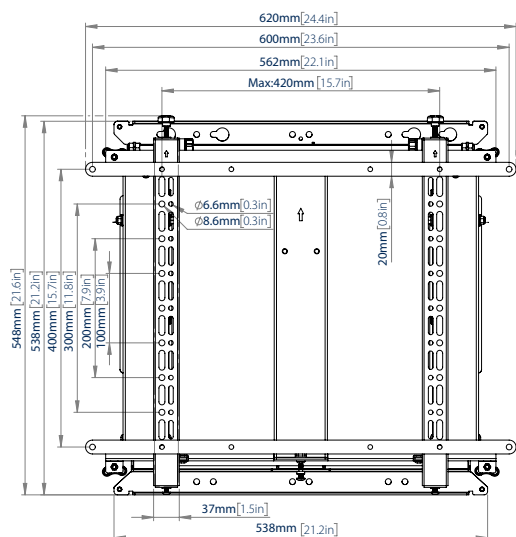
FRONT VIEW WITH ADAPTER ARMS
