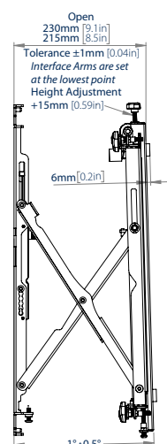
SIDE VIEW EXTENDED
